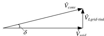
Fig. 2. Phasor diagram of voltage control grid-connection.
