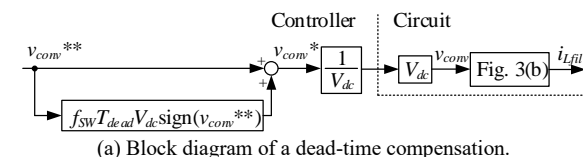
(a) Block diagram of a dead-time compensation.
