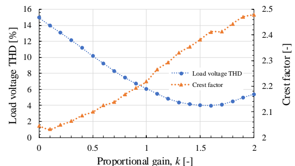
Fig. 13. Load voltage THD and crest factor characteristics with changing gain k .
