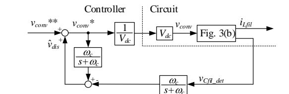
Fig. 4. Block diagram of the conventional semi-open-loop control.
