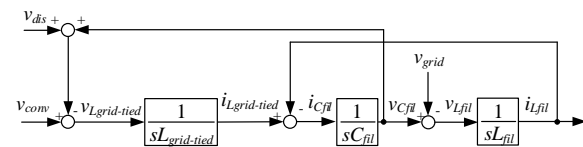
(b) Block diagram of a LCL filter with a power grid.
