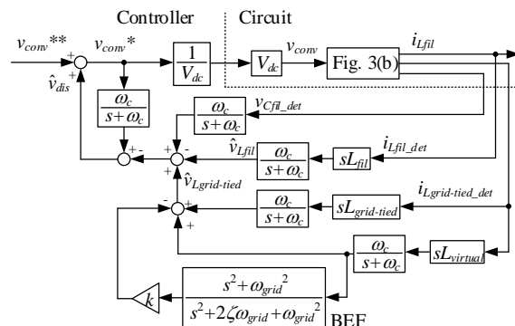
Fig. 5. Block diagram of proposed semi-open-loop control.
