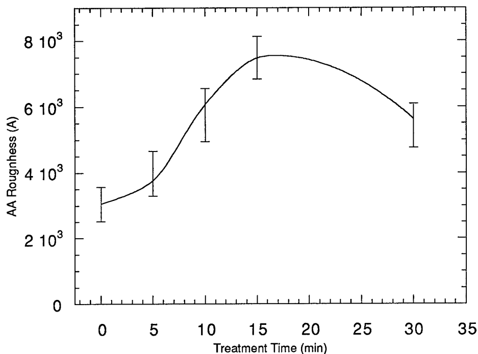
Figure 4.4: Arithmetic average roughness versus etching time
