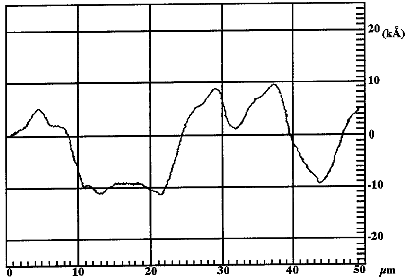
Figure 4.7: Typical profilometry scan for a sample etched for 30 minutes
