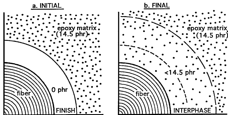
Figure 2.1: Schematic diagram of the interphase region: (a) initial bonding; (b) after final cure [55]
