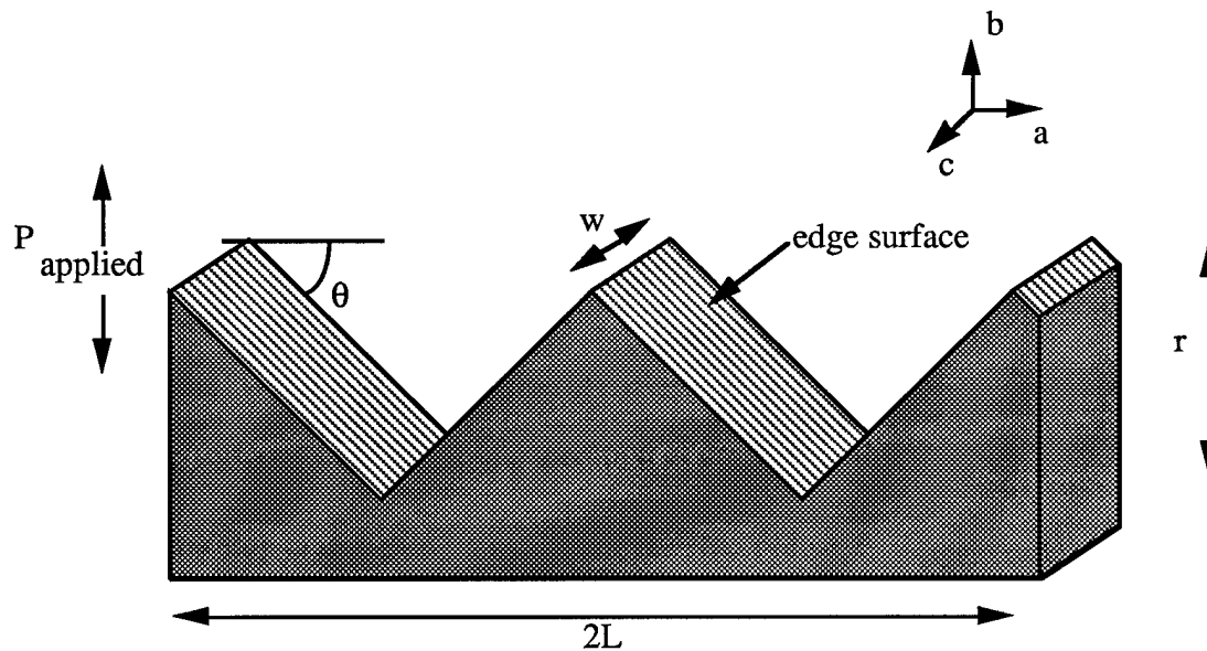
Figure 5.3: Idealized surface morphology of graphite substrates
