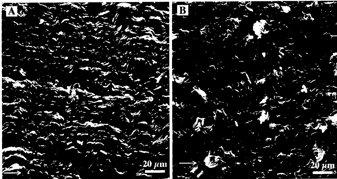
Figure 4.12: Fracture surfaces of an untreated specimen: (a) graphite side; (b) polymer side
