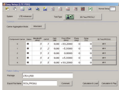
MX370108A LTE IQproducer / MX370108A-001 LTE-Advanced FDD Option LTE-Advanced Easy Setup画面例
