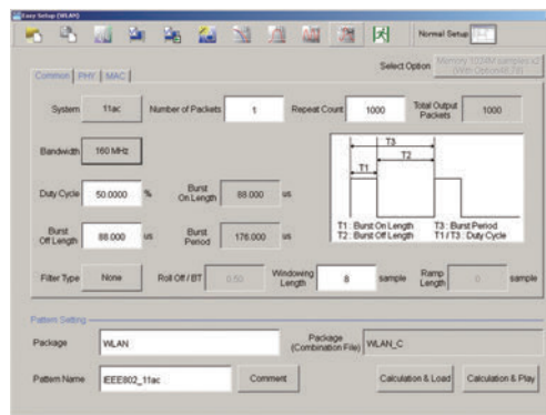
MX370111A WLAN IQproducer / MX370111A-002 802.11ac (160MHz) Option WLAN IEEE 802.11ac Easy Setup画面例
