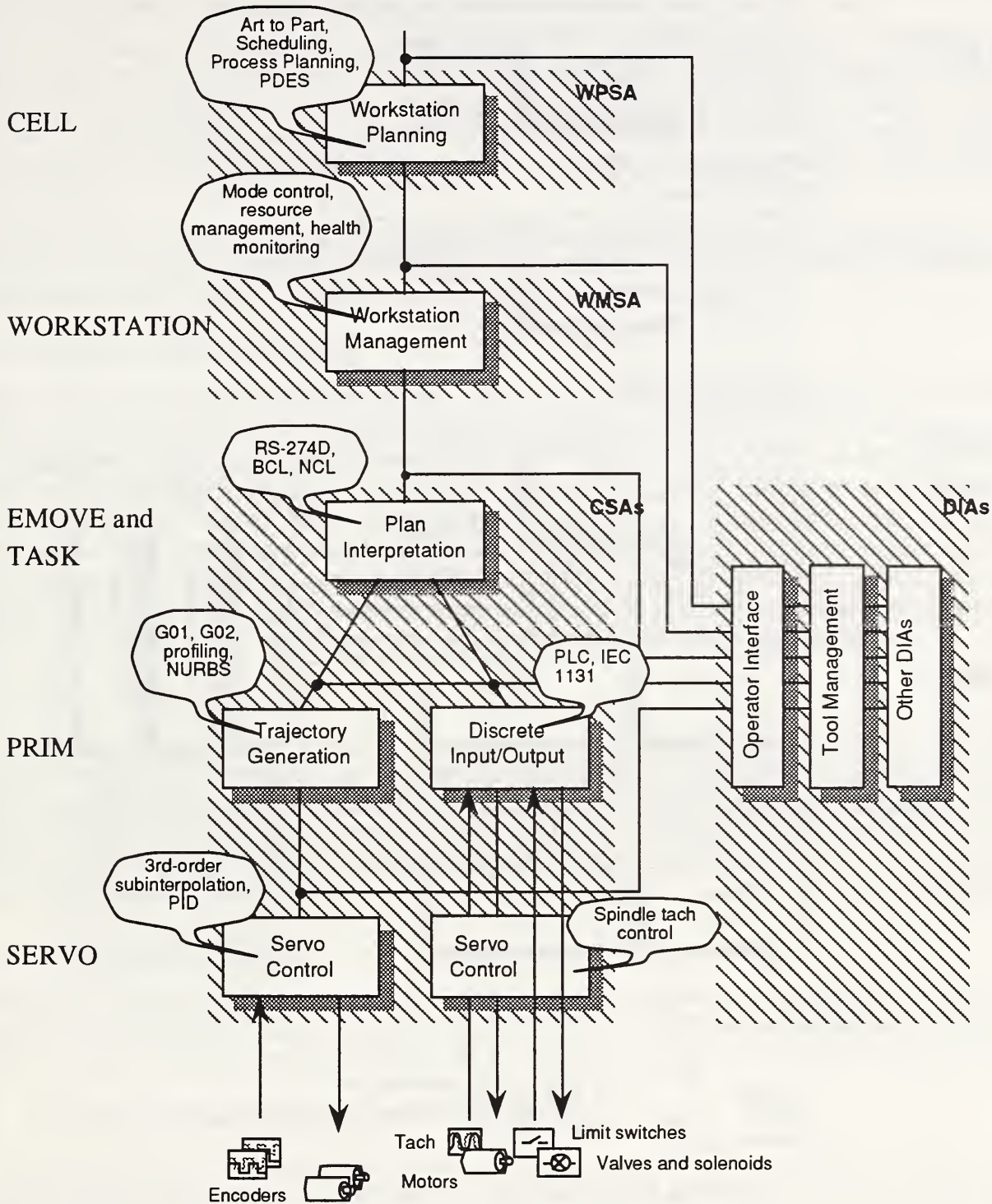
Figure 1. EMC Modules
