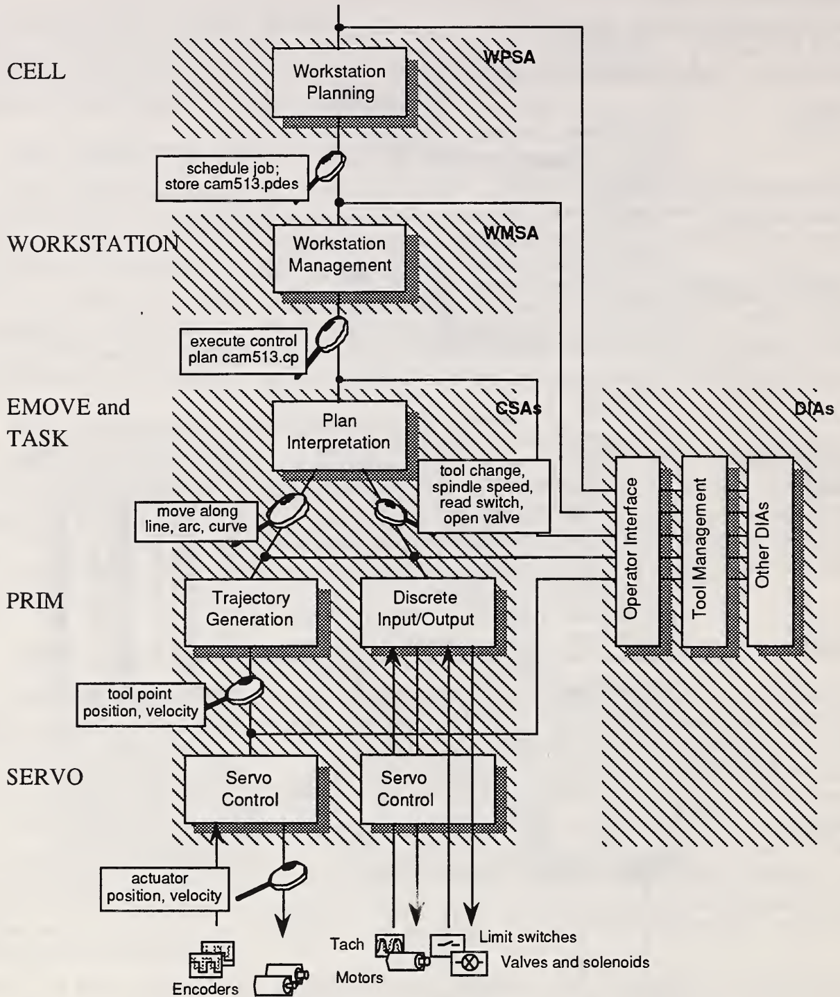
Figure 2. EMC Messages
