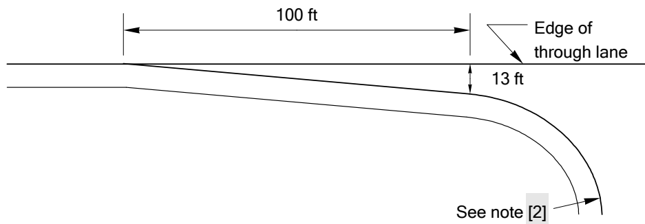
Right-Turn Taper
