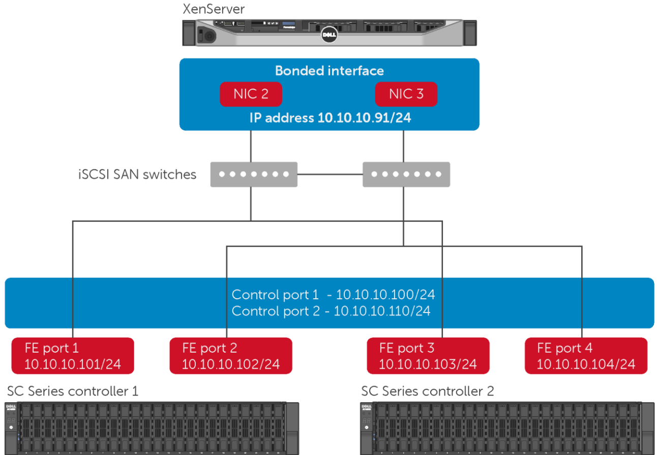
Figure 7 Open-iSCSI: single subnet and MPIIO
