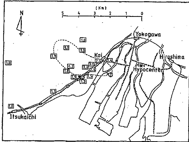
Fig. 6. The dashed line area indicates the distinct fallout area of Hiroshima atomic bomb over about 0.25 \text{ mC kg}^{-2} (1 R) of the cumulative exposure. The values in the square are the early survey data measured by Yamasaki (1953) representing the ratio of external radiation to natural background.
