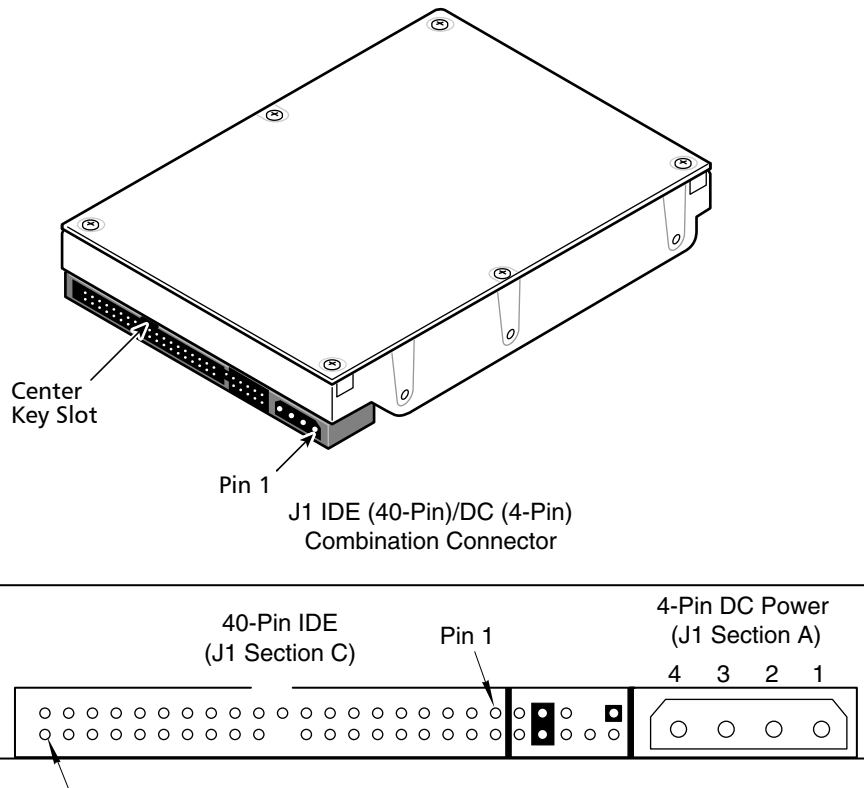
Figure 3-6 J1 DC Power and ATA Bus Combination Connector
