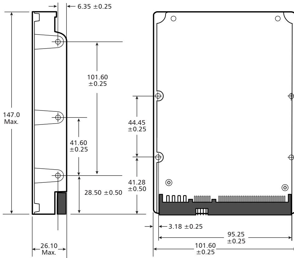
Figure 3-9 Mounting Dimensions for the MaXLine Plus II 250GB AT Hard Disk Drives
