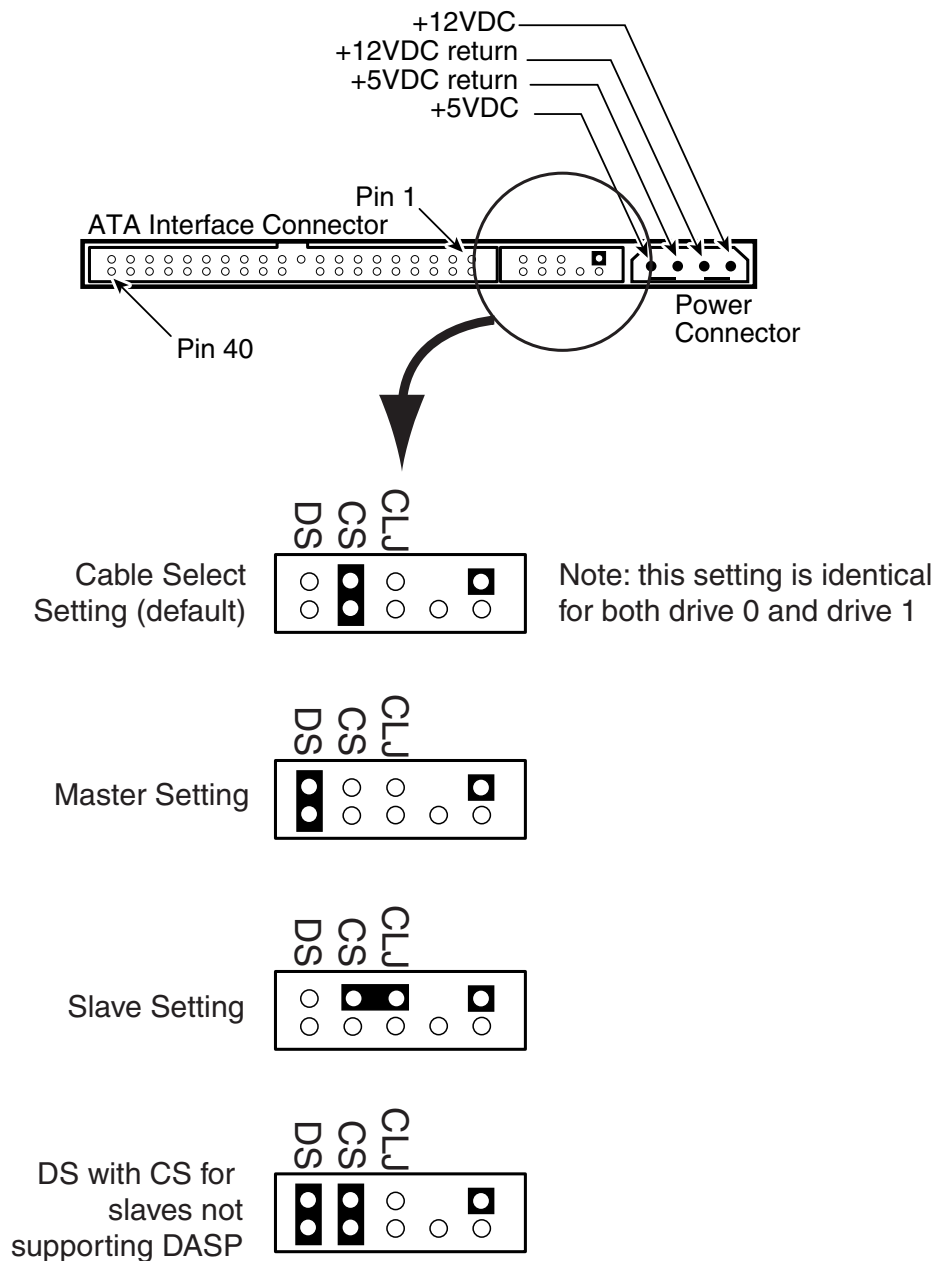
Figure 3-4 Jumper Locations on the ATA Interface Connector
