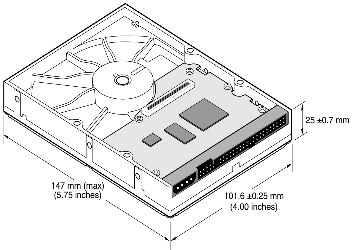
Figure 3-1 shows the external dimensions of the MaXLine Plus II 250GB AT drives.
