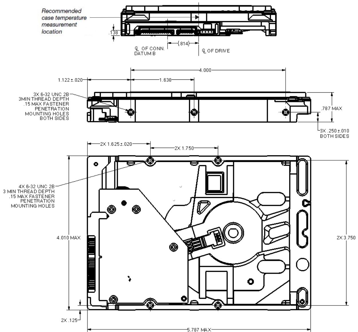
Figure 2 Mounting dimensions (1TB & 500GB models)
